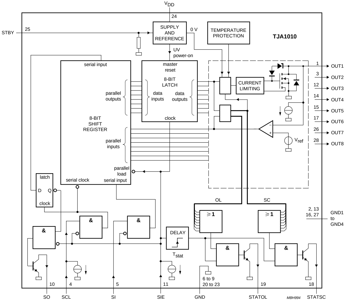
Fig.1 Block diagram.
